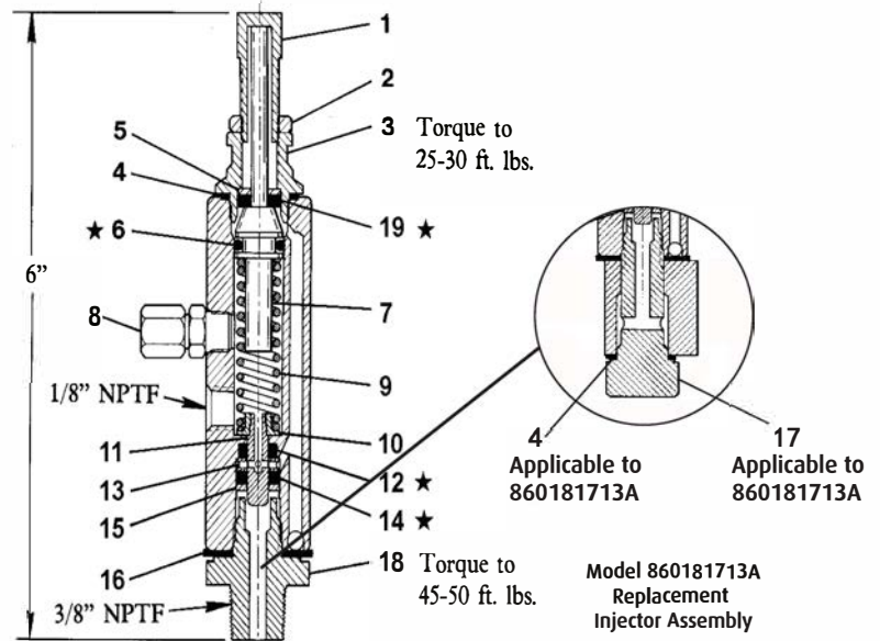
Model 860181713 Single Unit Injector
